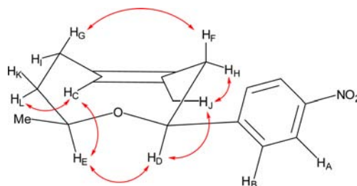
Figure 3. ^1\text{H} NMR NOESY of compound 9a .
