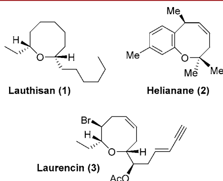
Figure 1. Structures of oxacyclic natural products.
