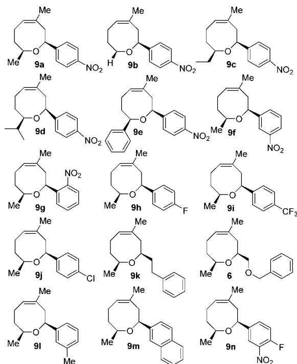
Figure 2. Structure of major isomer.
