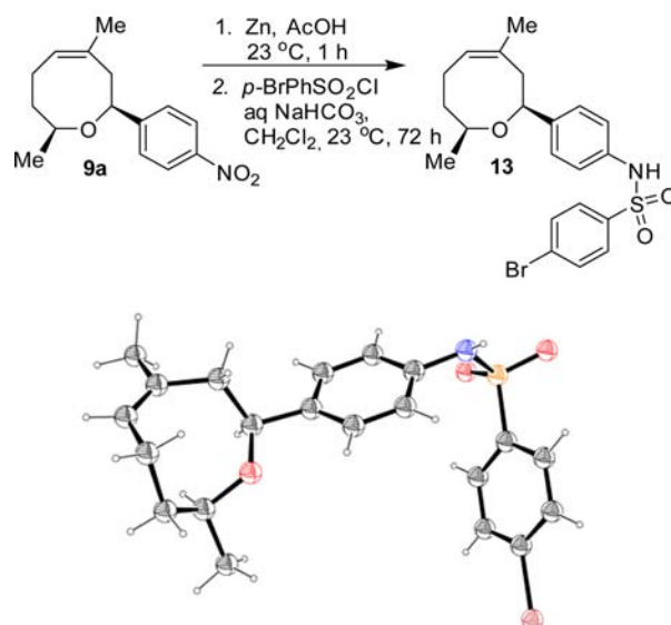
Scheme 4. Synthesis and X-ray Structure of 13 a
