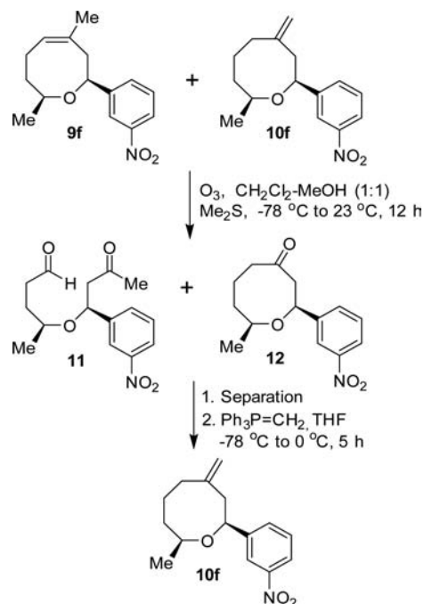
Scheme 4. Synthesis and X-ray Structure of 13 a
