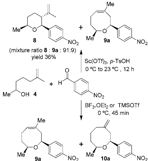
Scheme 2. Formation of Oxocene Products
