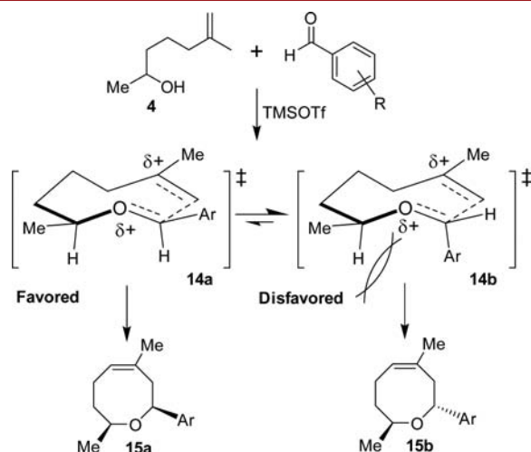
Figure 4. Stereochemical analysis for cis -oxocene products.
